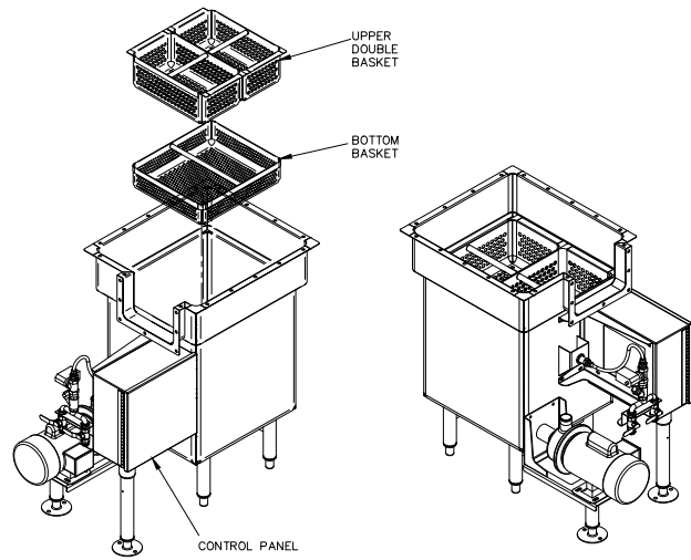
ISOMETRIC VIEWS
