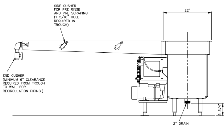
WASTE COLLECTOR DETAILS WITH TROUGH
